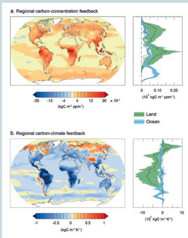
Figure 5: Maps of the changes in carbon uptake in kg of carbon/m 2 for:
